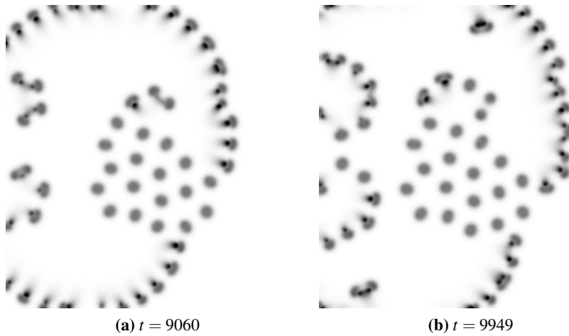
Figure 5.10: Two snapshots of the system resulting from equations 5.28–5.29, integrated on a surface of size 2 \times 2 with the parameters described in the text. The colours are adjusted so that the parasitic autocatalyst D , which forms into tails behind some of the spots, appears as a darker shade of grey than the primary autocatalyst B . A group of spots with tails can be seen on the left hand side of Plot (a), whereas in Plot (b) some tail-less spots can be seen in the same place, due to tails being lost during reproduction. The spots with tails move constantly away from their tails at a rate of approximately 4 \times 10^{-4} distance units per time unit, which results in their colonising the empty part of the space more rapidly than the tail-less spots. However, with this choice of parameters, spots with tails cannot invade areas colonised by tail-less spots, and the spots with tails are eventually crowded out and become extinct.
